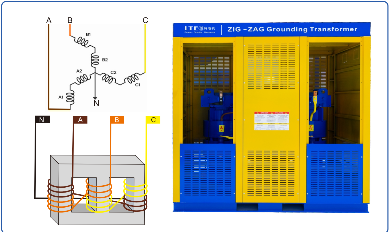
Zig-Zag Transformers
